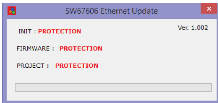
Figura 9: Ventana “Protection”
